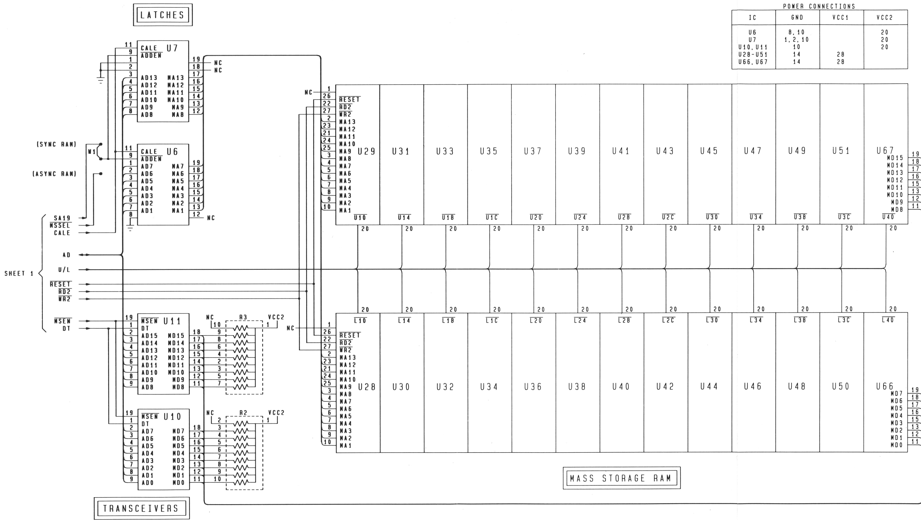
Figure 9-4. System PCA Schematic Diagram —Sheet 3
